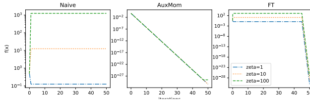
Figure 1: Effect of the bias \zeta (zeta in the figure) on the naive approach (Naive), AuxMom AuxMOM and Fine Tuning (FT) for K = 10, \delta = 1 and \eta = \min(1/2, 1/(\delta K)) . We can see that the naive approach fails to converge for big large bias values, whereas AuxMom AuxMOM converges all the time, no matter the value of the bias. Fine Tuning converges much slower (note the difference in scale) for small values of \delta , but beats AuxMOM for \delta = 10 .
