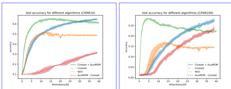
Figure 8: CIFAR10 and CIFAR100 experiments. Again, using AuxMOM leads to higher accuracy, similar to using the true dataset (W/O), whereas using the coreset alone leads to a loss in accuracy.
