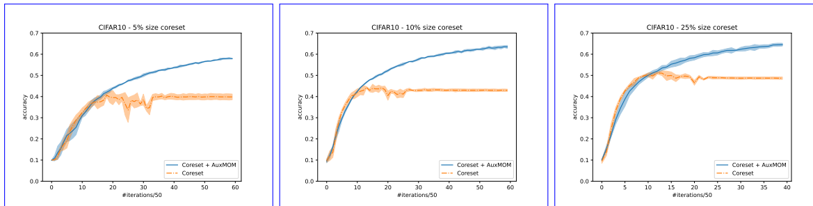
Figure 9: Effect of varying the coreset size on AuxMOM and pure coreset training. We see that the smaller the size of the coreset is, the worse the performance of training on the coreset alone; however, AuxMOM is only affected in terms of the number of iterations it needs to reach a given accuracy, which increases as the size of the coreset decreases.
