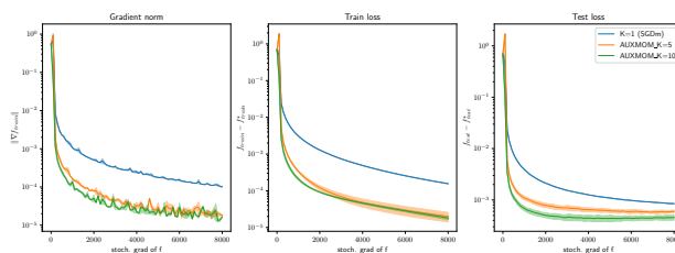
Figure 10: Gradient norm, train loss, and test loss. The We set the parameter a was chosen a = 0.1 , and the stepsizes were optimized using grid-search for best training loss.
