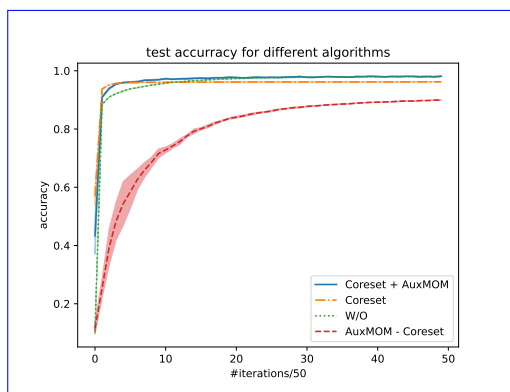
Figure 7: Comparing Coresets with and without AuxMOM. We see that with AuxMOM, we reach a higher accuracy, similar to using the true dataset (W/O).
