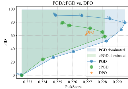
Figure 8: Reward-fidelity Pareto.
