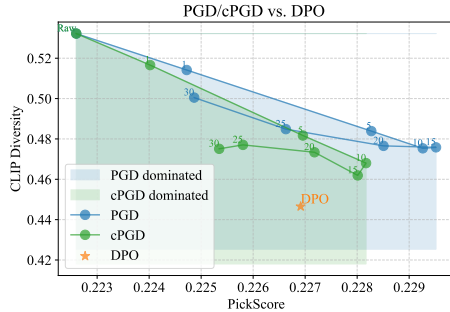
Figure 7: Reward-diversity Pareto.
