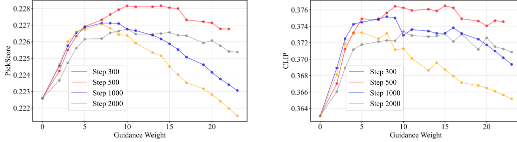
Figure 6: Effect of guidance weight w on automatic metrics (SDXL). Left: PickScore; Right: CLIP score. “Step” denotes the training steps of the guidance module. Curves rise quickly for small w ,
