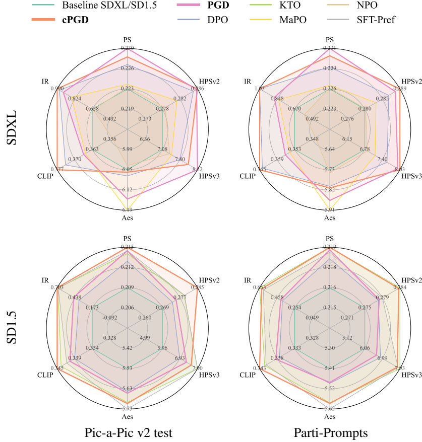
Figure 4: Overall comparison on SDXL (top) and SD1.5 (bottom). Radar axes report mean scores (higher is better): PickScore (PS), HPSv2, HPSv3, Aesthetics (Aes), CLIP, and ImageReward (IR). Polygons closer to the outer rim indicate better aggregate performance across metrics.
