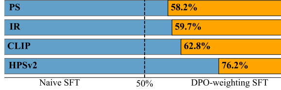
Figure 9: Comparison of SFT training with and without w_{\text{DPO}} weighting. Blue bars indicate naive SFT, and orange bars indicate weighted SFT. All results are obtained under the cPGD inference strategy with the same guidance weight.
