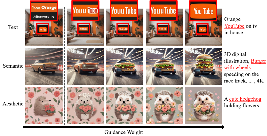
Figure 5: Qualitative effect of increasing guidance weight w (left \rightarrow right). Rows show text fidelity, semantic binding, and aesthetic style. Stronger w improves alignment and legibility up to a mid range, after which overshooting/rigidity appears.
