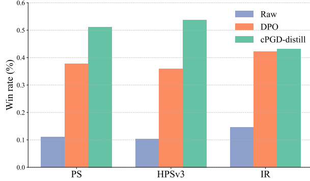
Figure 10: Win rate (%; higher is better) against the SDXL base across PickScore, HPSv3, and ImageReward. Bars show the proportion of prompts on which each method beats the base under the same random seeds. The distilled cPGD (500 steps) surpasses DPO on PickScore and HPSv3 and remains competitive on ImageReward.
