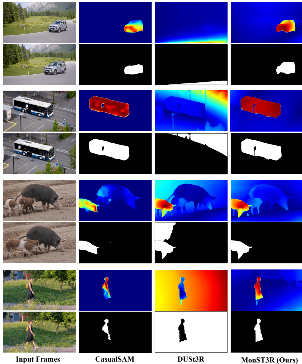
Figure A7: Qualitative comparison of static/dynamic mask. We visualize both the continuous error map (upper row) and binary static/dynamic mask (lower row). The threshold \alpha is fixed.
