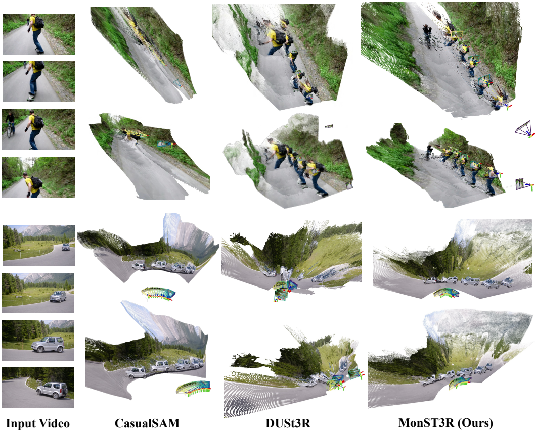
Figure 4: Qualitative comparison. Compared to CasualSAM and DUST3R, our method outputs both reliable camera trajectories and geometry of dynamic scenes. Refer to Fig. A5 for more results.
