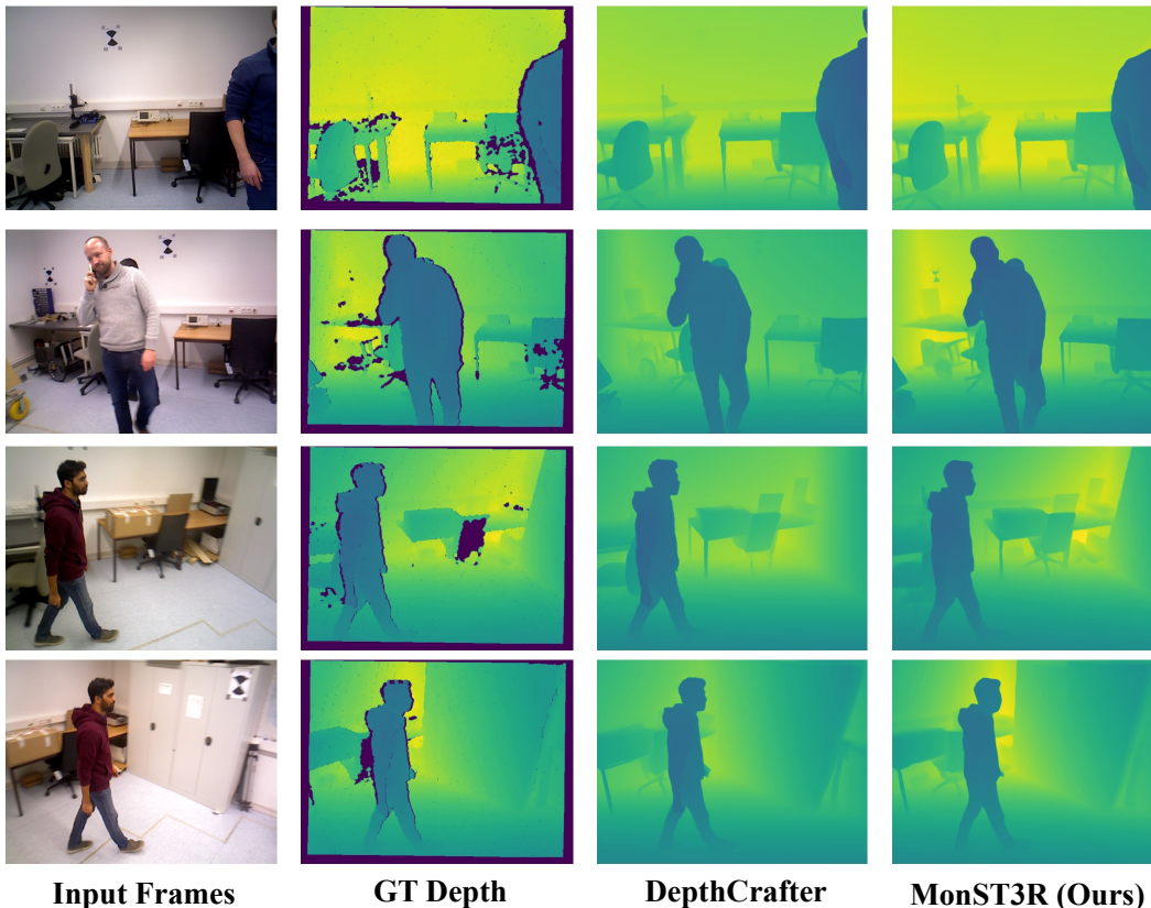
Figure A1: Video depth estimation comparison on Bonn dataset. Evaluation protocol is per-sequence scale & shift. We visualize the prediction result after alignment. Note, in the first row, our depth estimation is more aligned with the GT depth ( e.g. , the wall) compared to DepthCrafter’s.
