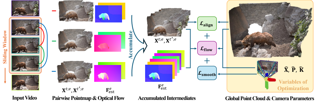
Figure 3: Dynamic global point cloud and camera pose estimation. Given a fixed sized of temporal window, we compute pairwise pointmap for each frame pair with MonST3R and optical flow from off-the-shelf method. These intermediates then serve as inputs to optimize a global point cloud and per-frame camera poses. Video depth can be directly derived from this unified representation.
