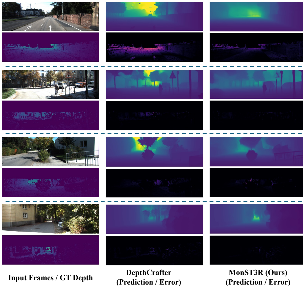
Figure A2: Video depth estimation comparison on KITTI dataset. Evaluation protocol is per-sequence scale & shift. For each case, the upper row is for input frame and depth prediction; the lower row is for ground truth depth annotation and error map. Prediction result is after alignment.
