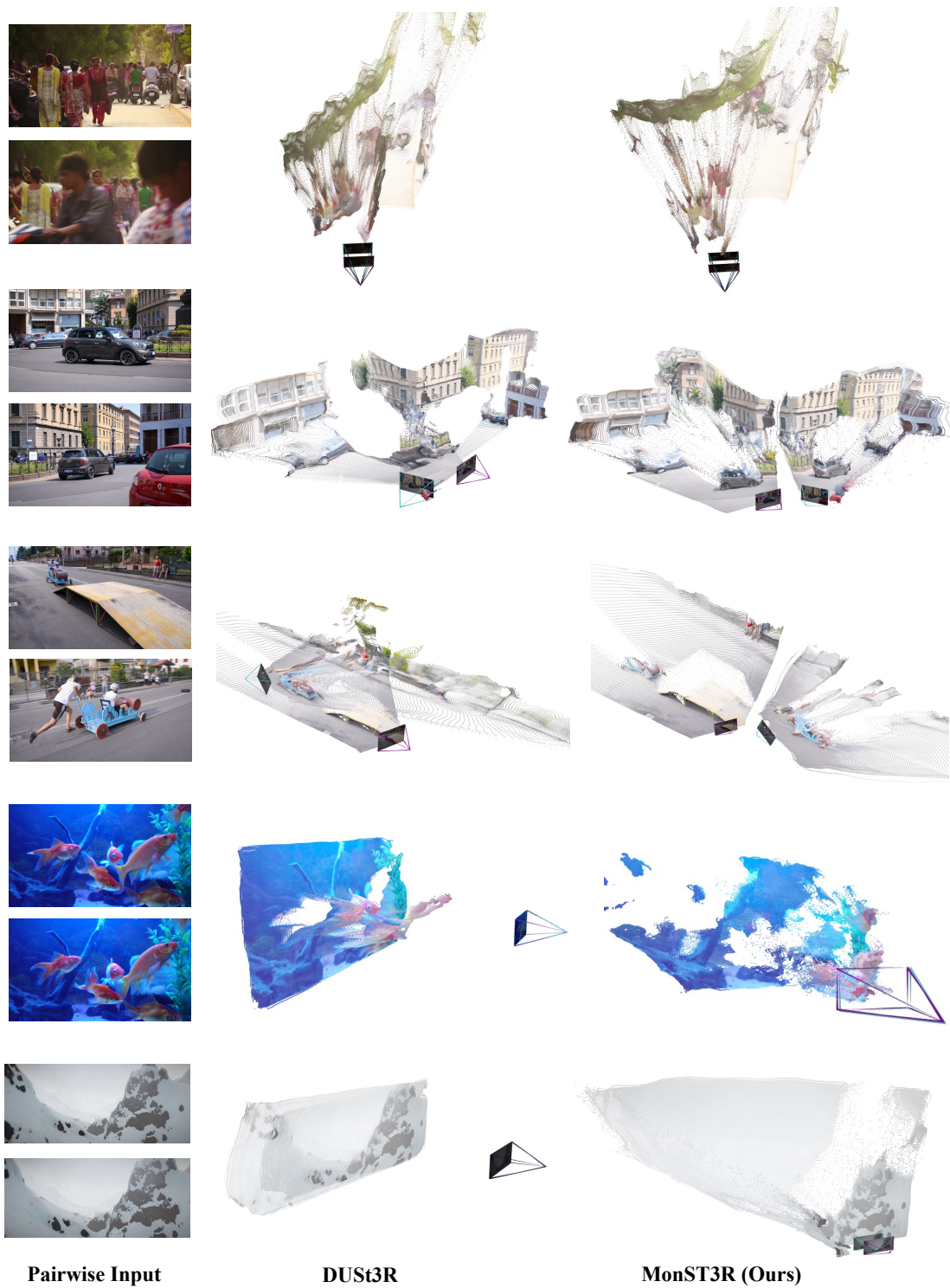
Figure A6: Qualitative comparison of feed-forward pairwise pointmaps prediction.
