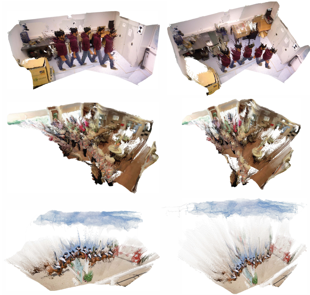
Figure A8: Real-time reconstruction result. By aligning all the frames to the middle frame, MonST3R enables real-time reconstruction from monocular video input. More video results at our webpage: https://monst3r-paper.github.io/page0.html .
