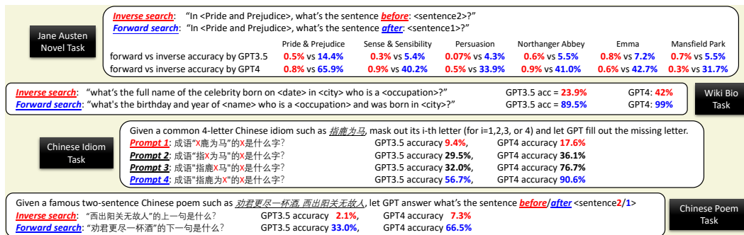
Figure 4: Forward search vs inverse search on ChatGPT (GPT3.5 / GPT-4); details in the full paper. (While inverse search may seem challenging even for humans, we have designed the Chinese idiom/poem tasks that are allegedly simple for many high school graduates in Chinese education.)
