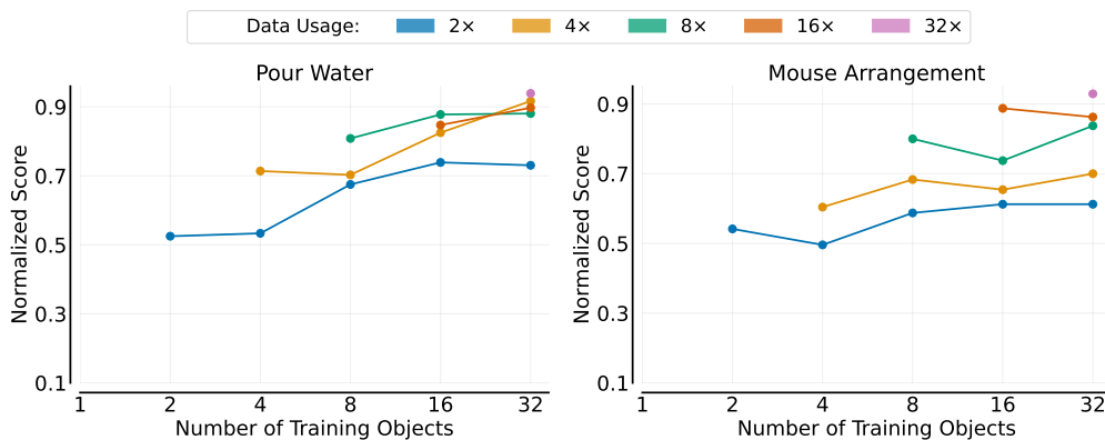
Figure 21: Object generalization. Each curve corresponds to a different total numbers of demonstrations used, with normalized scores shown as a function of the number of training objects.
