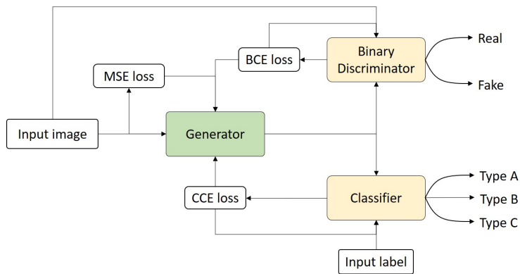
Figure 6: Extended Data Figure 3: Three-player architecture schematic
