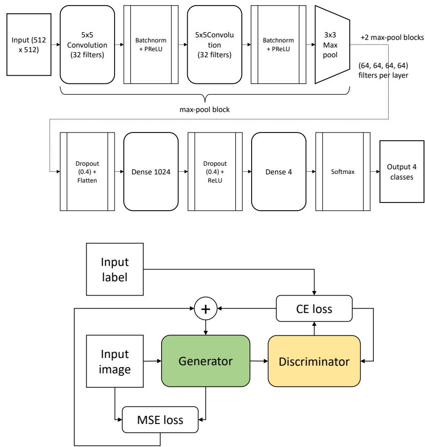
Figure 4: Extended Data Figure 1: Model Architecture. Top: layerwise architecture of our classifier, architecture initially from DeepDicomSort. Bottom: Depiction of the general structure for our GAN architecture.
