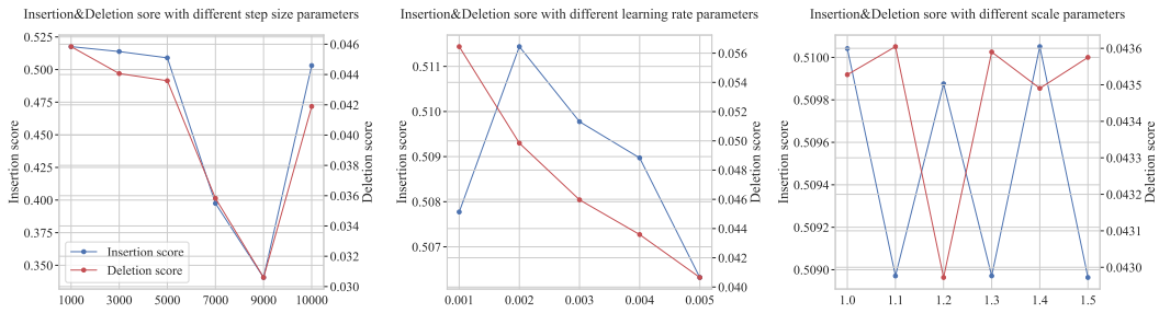
Figure 2: The ablation study of ISA on VGG_16
