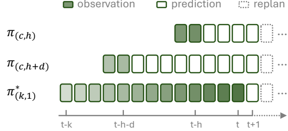
Figure 3: Illustration of (k, 1) -expert, (c, h) -learner, and (c, h + d) -learner. Shaded regions represent observed history; darker indicate greater influence on current decision.
