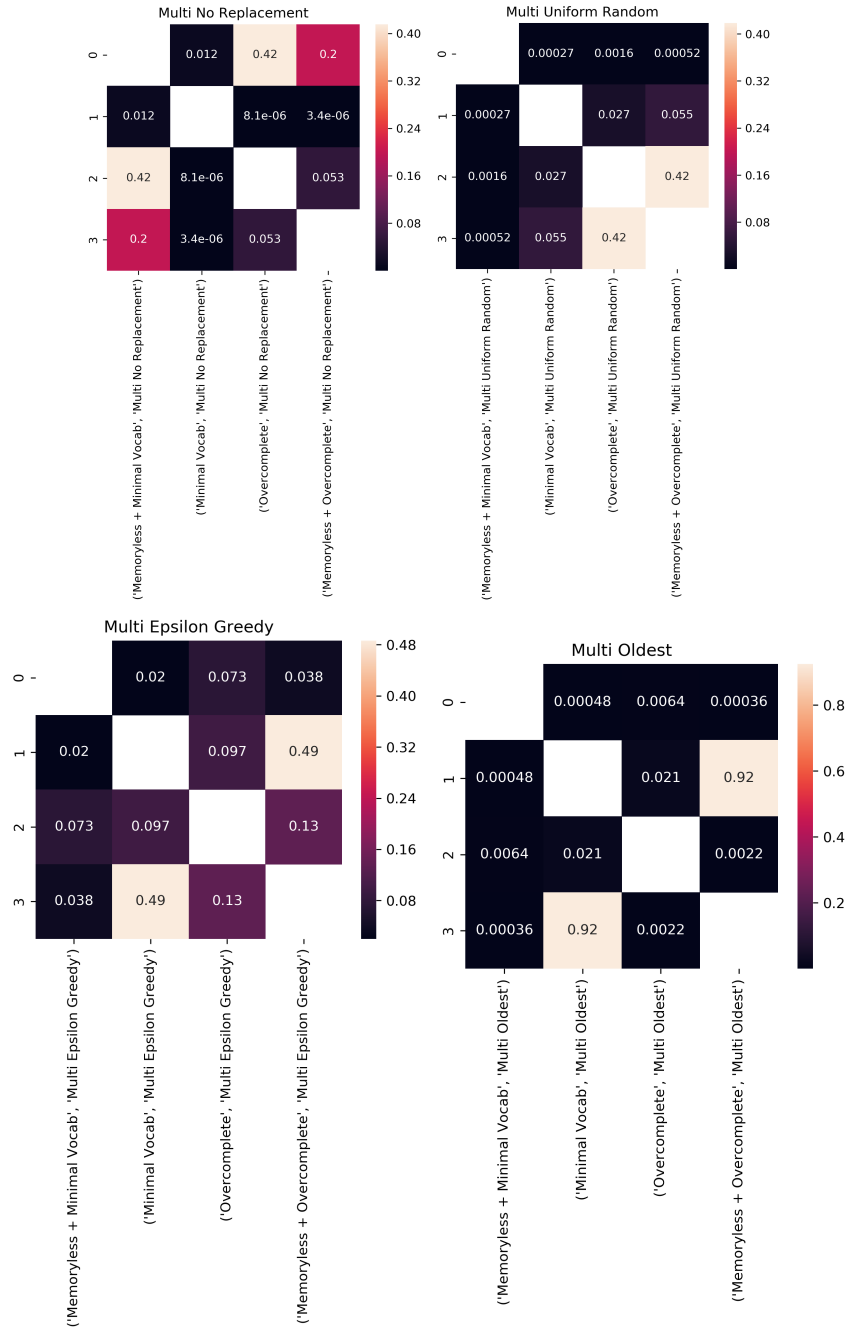
Figure 8: Multi Agent model comparison p-values.
