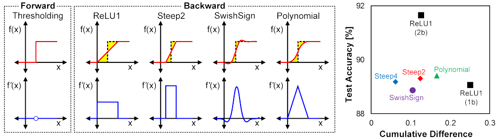
Figure 2: Activation functions and their derivatives used at forward and backward passes (left). The relationship between the best test accuracy and the cumulative difference of various STEs (right). Steep4 is extended version of steep2 with slope of 4.
