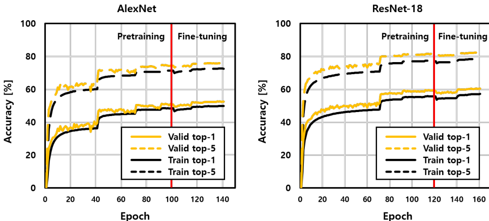
Figure 10: Training curves for AlexNet and ResNet-18 with BinaryDuo training scheme.
