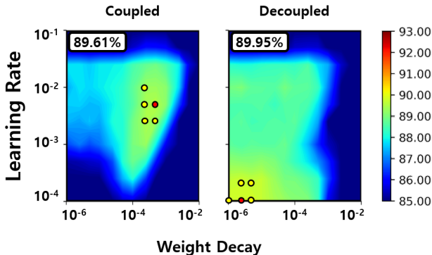
Figure 11: Training result of coupled 2-bit model and the corresponding decoupled model.
