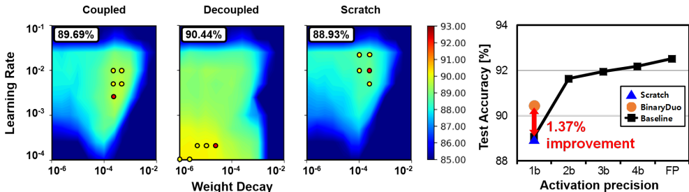
Figure 6: Training results of VGG-7 on CIFAR-10 dataset in the order of coupled ternary model, decoupled binary model and decoupled binary model trained from scratch (left). The best accuracy result is shown in the top left corner of each contour plot. Test accuracy of various models with different activation precision and training schemes (right).
