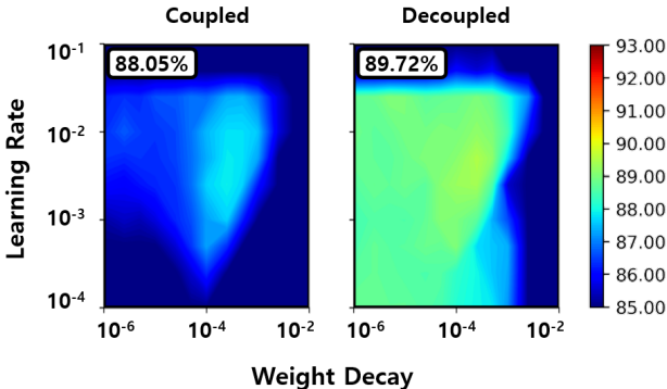
Figure 13: Training results of coupled ternary model and decoupled binary model when using BinaryDuo-Q.
