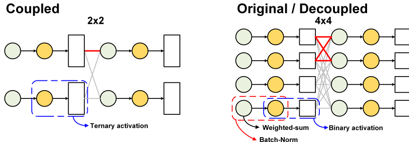
Figure 12: Example model architectures of coupled ternary and decoupled binary model when using BinaryDuo-Q. Coupled ternary model with 2x2 configuration is decoupled to binary model with 4x4 configuration.
