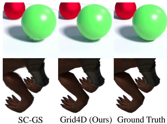
Figure 2. Qualitative comparisons to SC-GS on the synthetic D-NeRF dataset.
