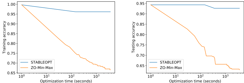
Figure 4: Comparison between ZO-Min-Max and STABLEOPT: training accuracy (left) or testing accuracy (right) versus optimization time.
