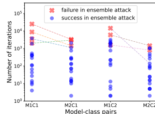
Figure 2: Success or failure of our ensemble attack versus successful per-image PGD attack.
