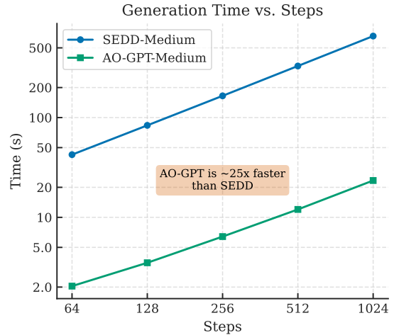
Figure 5. Generation time versus number of generation steps with sequence length 1024 and batch size= 32 for decoder-only AO-AR models (with KV-cache and Lemma 5.1) and their encoder-only counterparts (SEDD).
