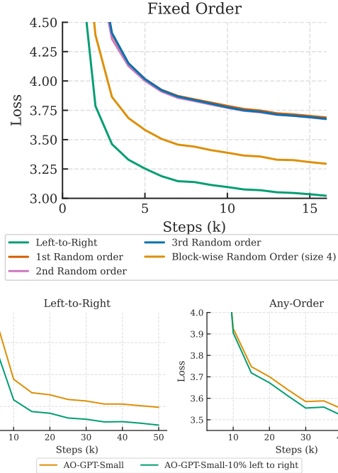
Figure 3. (a) Convergence speed with different fixed prediction orders: left-to-right, fixed random, and fixed block-wise random. (b) Impact of adding 10% left-to-right (L2R) data to AO-GPT training on its L2R and any-order loss.
