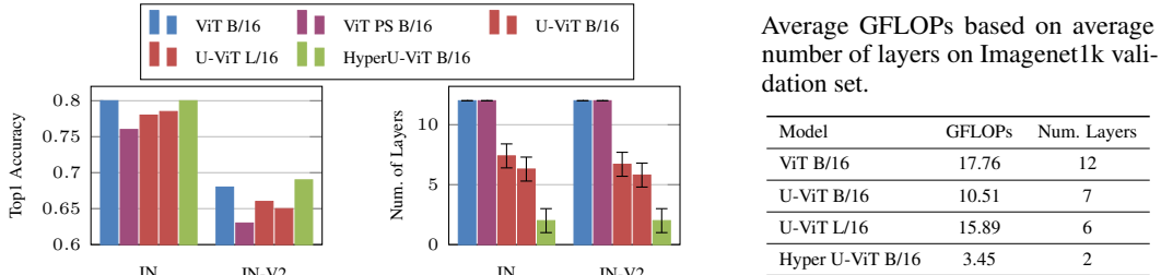
Figure 6: Performance of vision transformer models trained on ImageNet1k on ImageNet v1 and ImageNet v2 validation sets.
