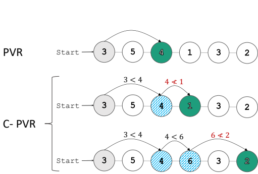
Figure 1: Example of PVR and C-PVR Tasks. In the regular PVR task, only one part of the input (in this case, the first element in the sequence) serves as the pointer. However, in the C-PVR, each element can act as a pointer. The task is to recursively retrieve the values until a condition is met. For this illustration, the condition is to continue as long as the sequence progresses forward. In this diagram, gray circles refer to initial steps, blue to intermediate steps, and green the final steps (the value of the green circle is returned).
