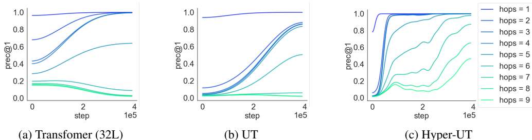
Figure 4: Implicit curriculum of transformers on C-PVR task. The y-axis is the accuracy and the x-axis is the training steps. This plot shows that transformers (a Hyper-UT instance) is learning examples in order of their complexity.
