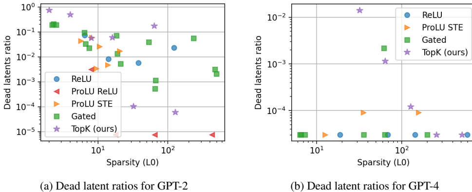
Figure 12: Our baselines generally have few dead latents, similar or less than our TopK models.
