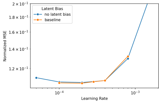
Figure 15: b_{enc} does not strongly affect loss (gpt2sm 128k, k=32).
