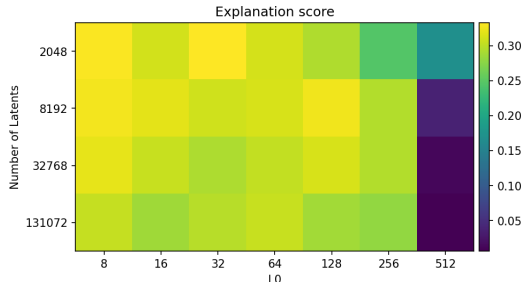
Figure 19: Explanation scores for GPT-2 small autoencoders of different n and k , evaluated on 400 randomly chosen latents per autoencoder. It is hard to read off trends, but the explanation score is able to somewhat detect the dense solutions region.
