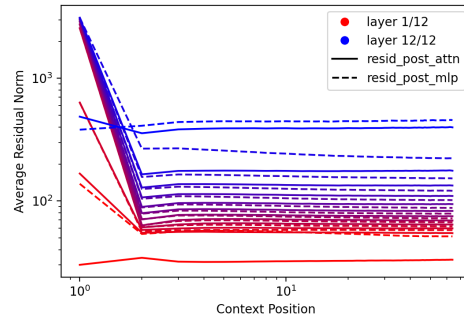
Figure 30: Residual stream norms by context position. First token positions are more than an order of magnitude larger than other positions, except at the first and last layer for GPT-2 small.
