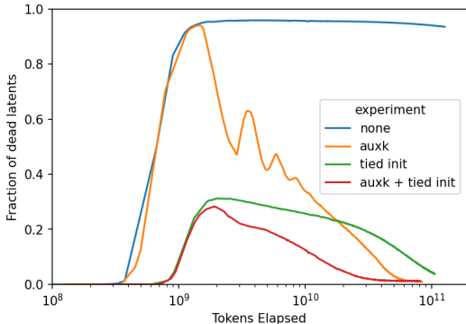
Figure 13: Methods that reduce the number of dead latents (gpt2sm 2M, k=32). With AuxK and/or tied initialization, number of dead latents generally decreases over the course of training, after an early spike.
