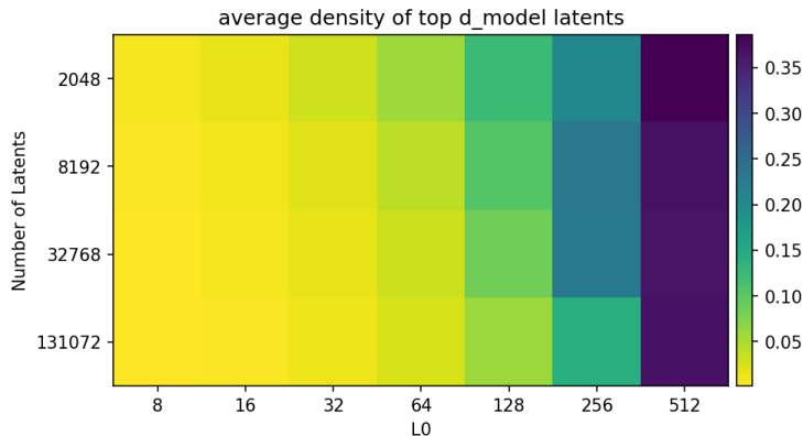
Figure 18: Average density of the d_{model} most-dense features, divided by L_0 , for different autoencoders. When k = 512 , the learned autoencoders have many dense features. This corresponds to when ablations stop having sparse effects subsection 4.5, and anecdotally corresponds to noticeably less interpretable features. For k = 256, n = 2048 , there is perhaps an intermediate regime.
