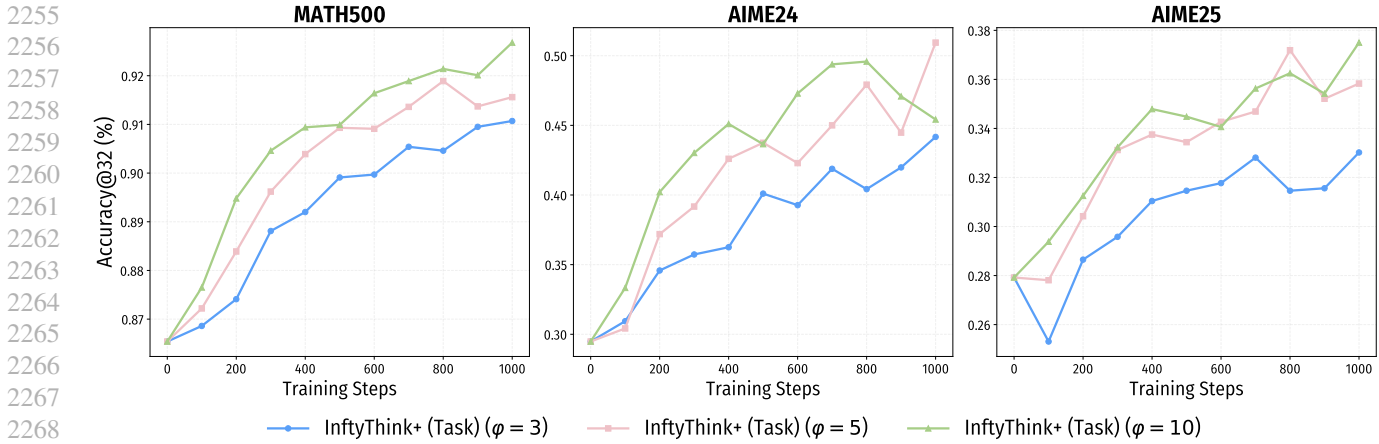
(a) Evaluation trajectories of InftyThink+ trained with task reward only under different iteration caps \varphi \in \{3, 5, 10\} .
