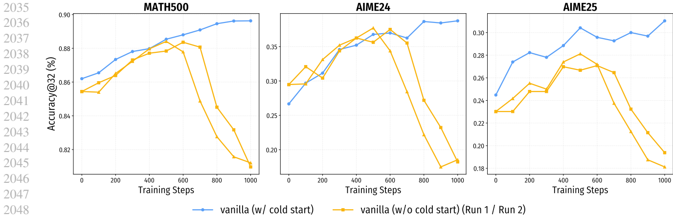
Figure 17. Benchmark performance along training for vanilla RL with vs. without cold start.
