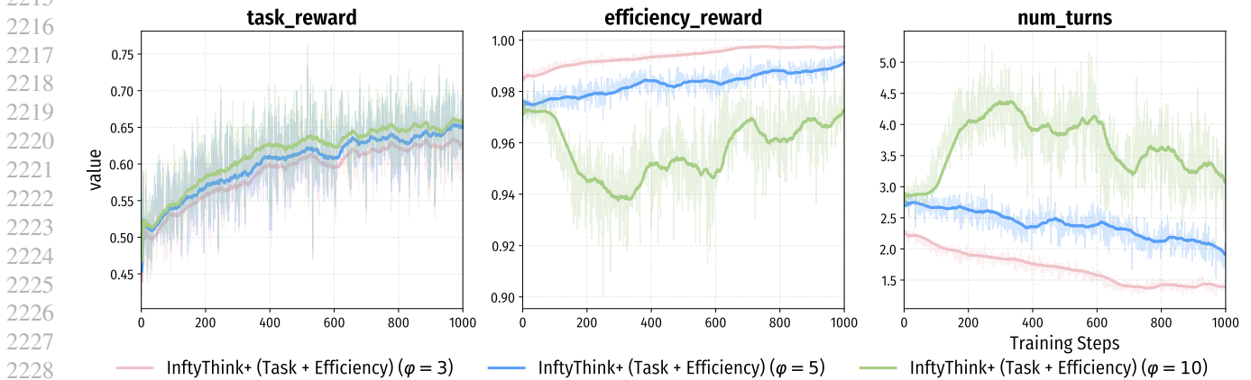
(b) InftyThink-related metrics of InftyThink+ trained with task + efficiency rewards under different iteration caps \varphi \in \{3, 5, 10\} .
