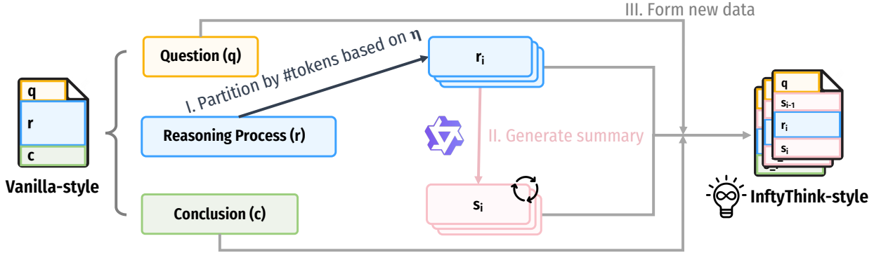
Figure 6. Systematic pipeline for reconstructing vanilla-style long-context reasoning data into the InftyThink-style format. I. Original reasoning processes are partitioned into optimally sized fragments based on parameter ( \eta ), preserving semantic coherence. II. Qwen3-4B-Instruct-2507 generates concise yet comprehensive summaries for each reasoning fragment. III. The original fragments and their generated summaries are systematically recombined to create InftyThink-style training instances that teach the model to reason iteratively. We adopt the figure design style from Yan et al. (2025).
