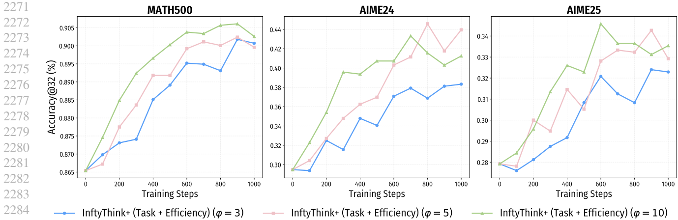
(b) Evaluation trajectories of InftyThink+ trained with task + efficiency rewards under different iteration caps \varphi \in \{3, 5, 10\} .
