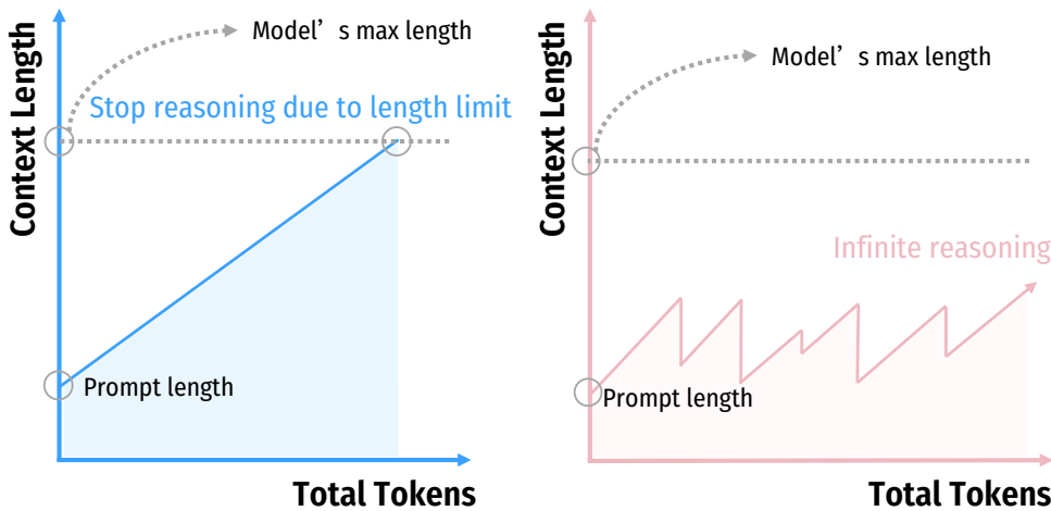
Figure 5. Computational complexity comparison between vanilla long-context reasoning (blue, left) and InftyThink (pink, right). The sawtooth pattern of InftyThink demonstrates how periodic summarization creates a bounded memory footprint, substantially reducing computational costs (smaller area under curve) while enabling deeper reasoning. We adopt the figure design style from Yan et al. (2025).
