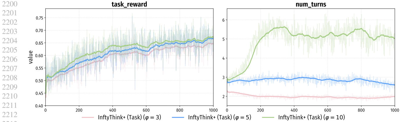
(a) InftyThink-related metrics of InftyThink+ trained with task reward only under different iteration caps \varphi \in \{3, 5, 10\} .
