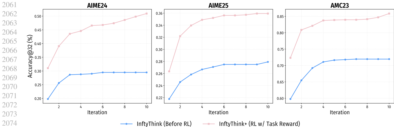
Figure 18. Accuracy across of reasoning iterations. We report Accuracy@32 on AIME24, AIME25, and AMC23 when allowing the model to perform up to j InftyThink-style reasoning rounds (x-axis), where each round is connected by the model-generated summary.
