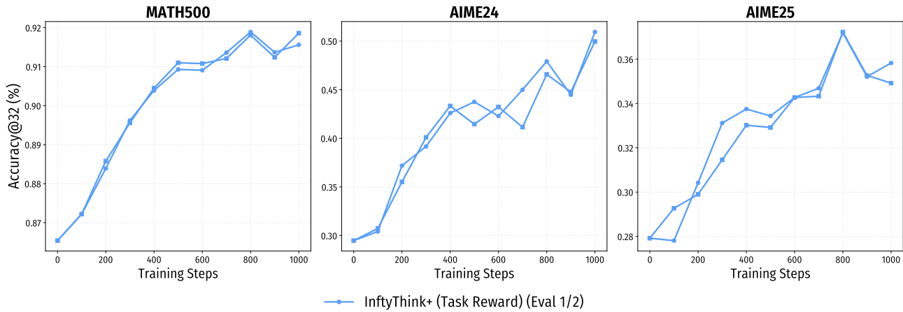
Figure 15. Evaluation stability across repeated runs.
