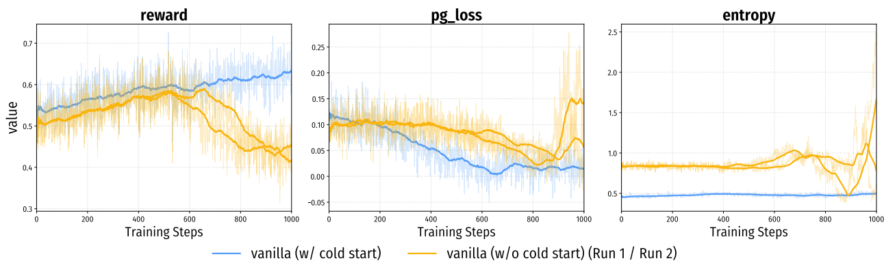
Figure 16. Training dynamics of vanilla RL with vs. without cold start.
