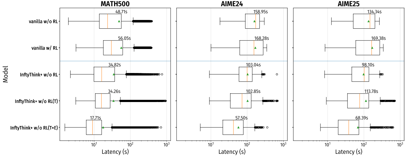
Figure 19. Inference latency distribution on MATH500, AIME24, and AIME25 (log-scale x-axis). Each row corresponds to one model variant. Boxes denote the interquartile range (IQR) with the median marked in orange; green triangles indicate the mean; whiskers extend to 1.5 \times \text{IQR} ; dots are outliers. InftyThink+ shifts the distribution left and suppresses the long-latency tail, while adding the efficiency reward (RL(T+E)) yields the largest latency reduction.
