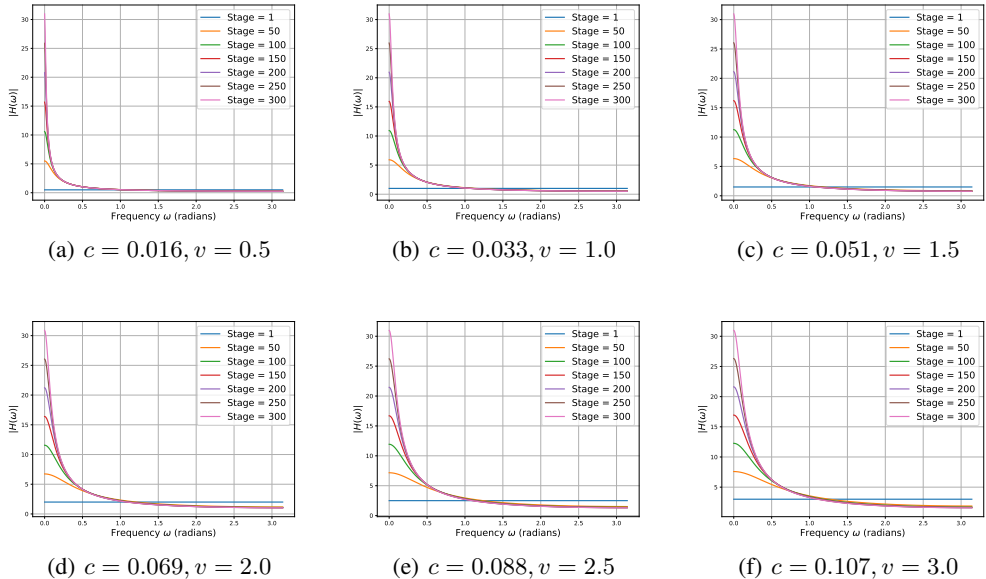
Figure 13: The dynamic magnitude responses of the black points in the optimal zone.
