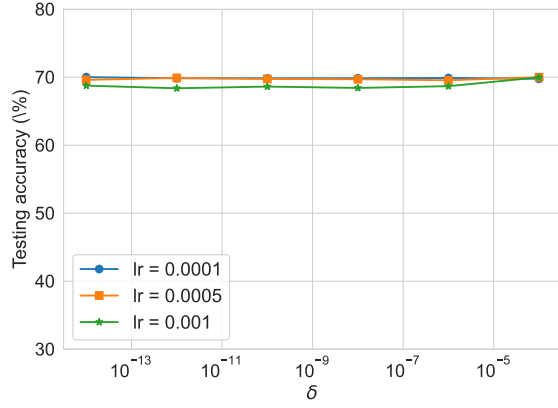
Figure 2: Hyperparameter \delta robustness for ResNet18 on ImageNet.
