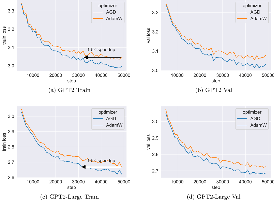
Figure 1: Training/validation loss of GPT2 (124 M) and GPT2-Large (774 M) on OpenWebText
