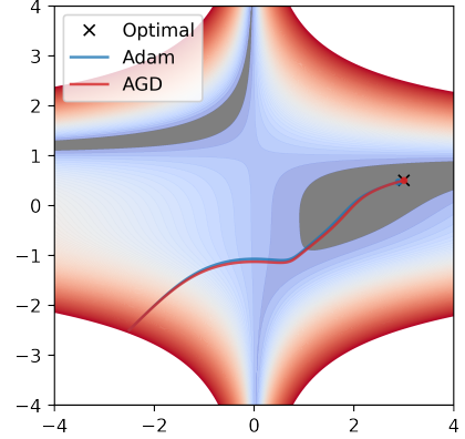
Figure 3: The whole optimization trajectories of AGD and Adam of Beale function.
