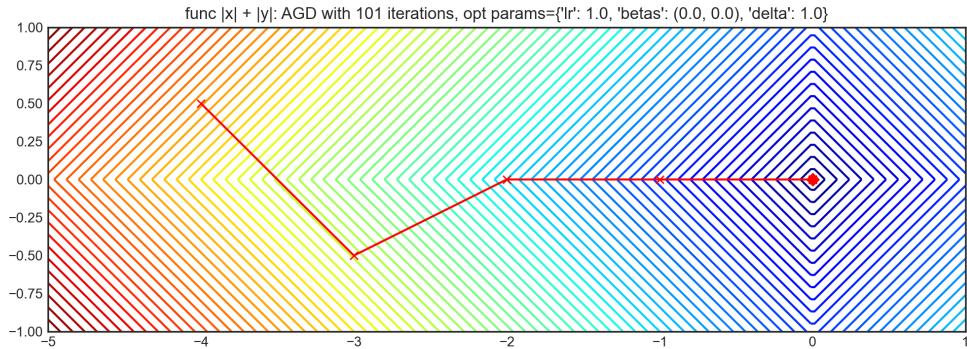
Figure 4: Optimize the function f(x, y) = |x| + |y| using AGD from the starting point (-4, 0.5) .
