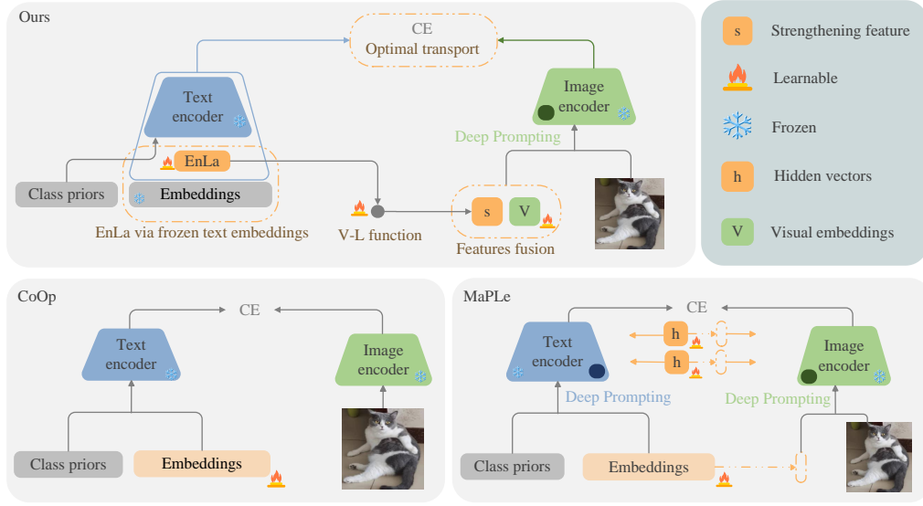
Figure 2: EnPrompt (Ours) aims to connect the image and text encoders by a novel design, which introduces the strengthening feature of the EnLa to fuse the learnable visual embeddings of the first layer of image encoder, while frozen text embeddings. Both CoOp and MaPLe employ designs to learn text embeddings. In our method, the fusion embeddings are further introduced in transformer of the image encoder for deep prompting.
