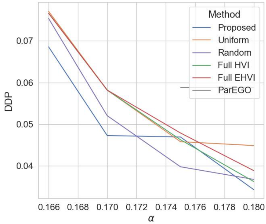
(a) Fairness
