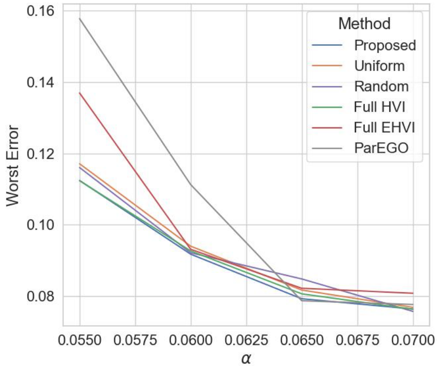
(b) Robustness
