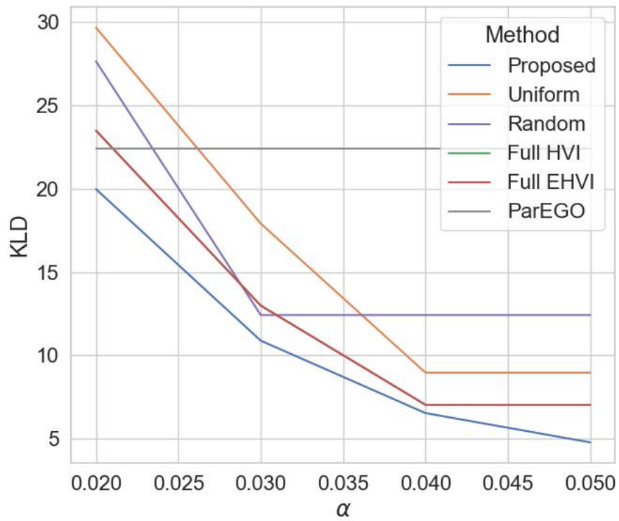
(c) VAE
