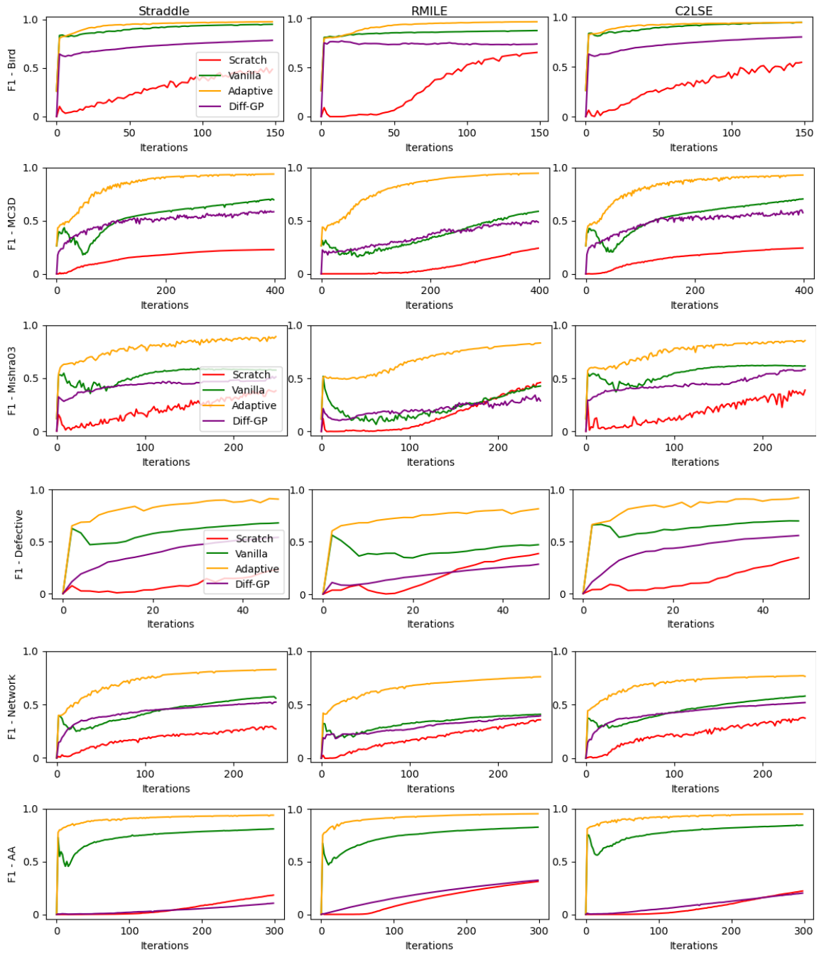
Figure 5: Transfer learning for active LSE with IMQ kernel
