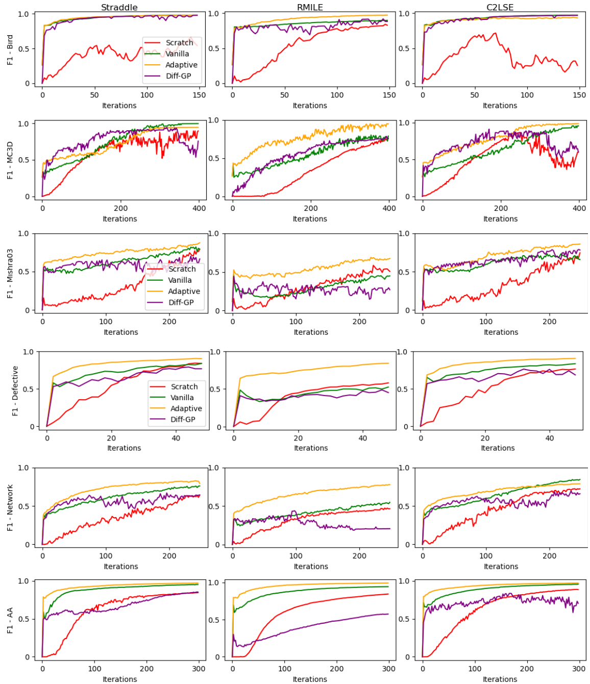
Figure 4: Transfer learning for active LSE with RBF kernel
