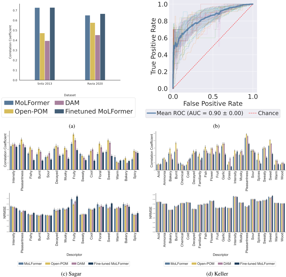
Figure III: Results including fine-tuned MoLFormer for (a) similarity ratings, (b) labels classification and (c,d) perceptual rating prediction.
