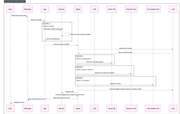
Figure 2. Sequence Diagram.
