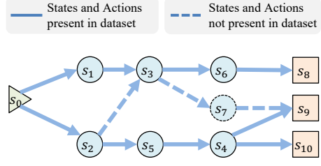
Figure 2: Illustration of supported and unsupported flows. Edges not presenting in the dataset are defined as unsupported flows. For instance, (s_2 \rightarrow s_3) is unsupported.
