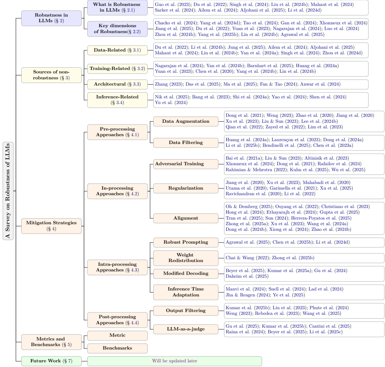
Figure 1: The outline of the survey on robustness of large language models.
