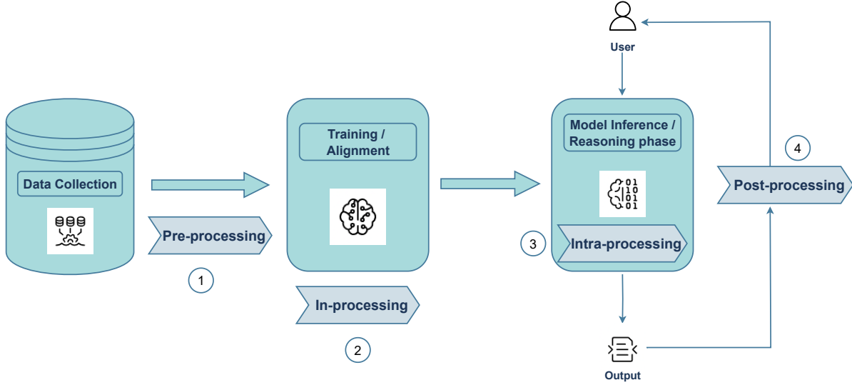
Figure 4: The robustness of Large Language Models (LLMs) can be systematically fortified through a layered pipeline. Beginning with data collection and annotation, diverse datasets and rigorous labelling establish a foundational resilience. Pre-processing strategies then clean, augment, and balance the data to mitigate biases and noise. During training and fine-tuning, in-processing techniques like adversarial learning and alignment strategies address vulnerabilities directly. As part of inference, intra-processing strategies dynamically adjust inputs (e.g., sanitising adversarial queries) to counter real-time risks. Finally, post-processing safeguards act as a last layer, refining outputs via alignment checks and ethical filters to ensure reliability. Together, these stages create a unified defence, ensuring adaptability and resilience across the LLM lifecycle.
