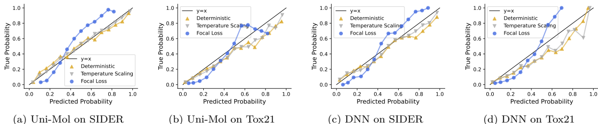
Figure 3: The calibration plot of UQ methods. Here “true probability” refers to the empirical prediction accuracy, and “predicted probability” refers to the average predicted probability within each bin. These results reveal that Temperature Scaling typically enhances calibration effectiveness in the majority of scenarios, whereas Focal Loss tends to lead to over-calibration of the model, producing under-confident results.
