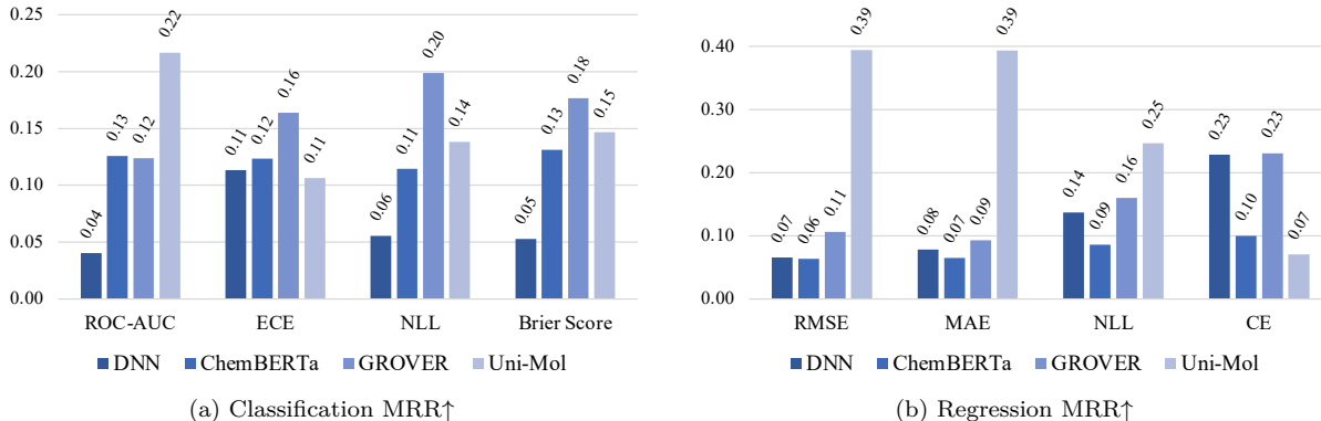
Figure 2: MRR of the backbone models; each metric is macro-averaged from the reciprocal ranks of all corresponding UQ methods across all datasets. Uni-Mol stands out by consistently surpassing its counterparts in property prediction accuracy for both classification and regression tasks. Conversely, GROVER exhibits a more balanced performance in both prediction accuracy and UQ across various tasks.
