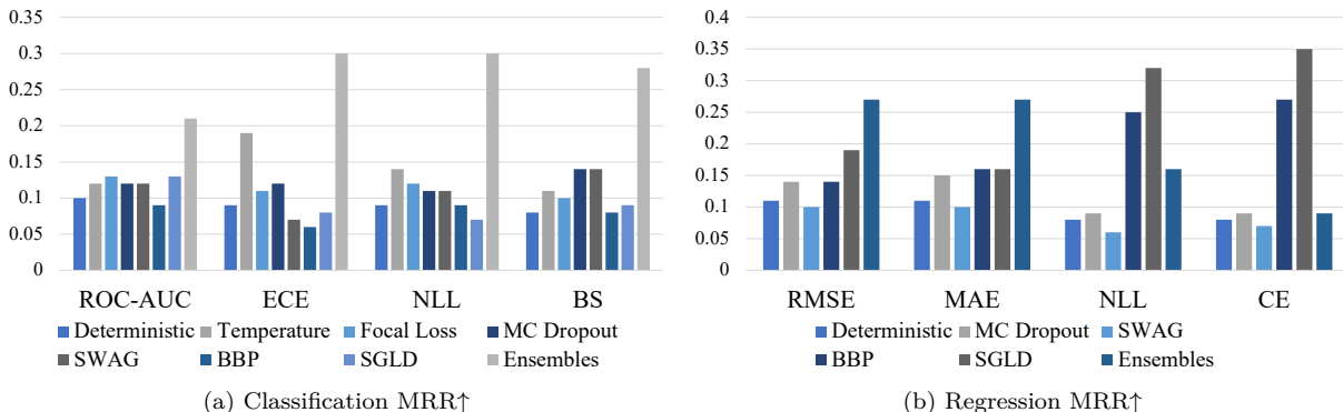
Figure 6: MRR of the UQ methods for each metric, each is macro-averaged from the reciprocal ranks of the results of all corresponding backbone models on all datasets.
