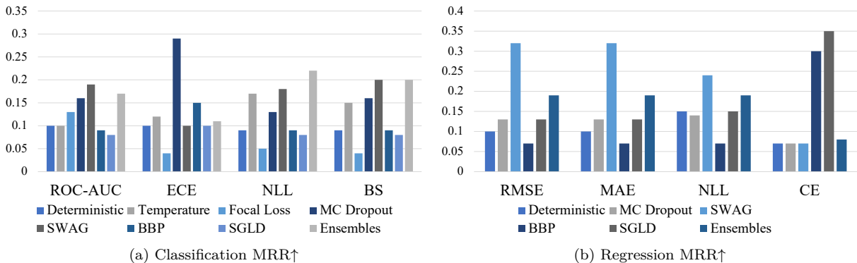
Figure 7: MRR of the UQ methods for each metric, each is macro-averaged from the reciprocal ranks of the results of all corresponding backbone models on all randomly split datasets.
