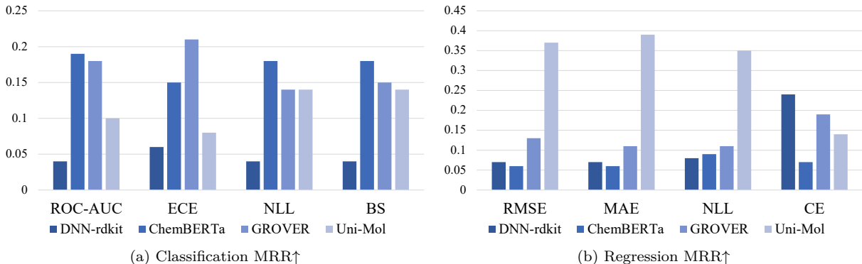
Figure 8: MRR of the UQ methods for each backbone model, each is macro-averaged from the reciprocal ranks of the results of all corresponding UQ methods on all randomly split datasets.
