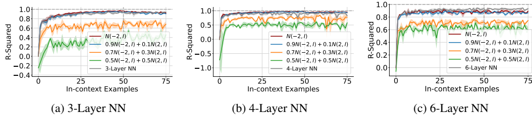
Figure 2: Performance of ICL in Softmax-Transformer: ICL learns 3-layer, 4-layer, and 6-layer NN and achieves R-squared values comparable to those from training with prompt samples. The results also show the ICL performance declines as the testing distribution diverges from the pretraining one. Note that performance decreases when the prompt length exceeds the pretraining length (i.e., 50), a well-known issue (Dai et al., 2019; Anil et al., 2022). We believe this is due to the absolute positional encodings in GPT-2, as noted in (Zhang et al., 2023)
