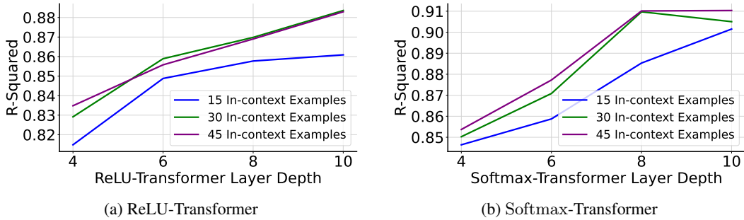
Figure 3: Performance of ICL Across Varying Transformer Depths: We use the number of in-context examples as 15, 30, or 45 for both the ReLU-Transformer and the Softmax-Transformer. The results show that a deeper transformer achieves better ICL performance, supporting the idea that scaling up the transformer enables it to perform more ICGD steps.
