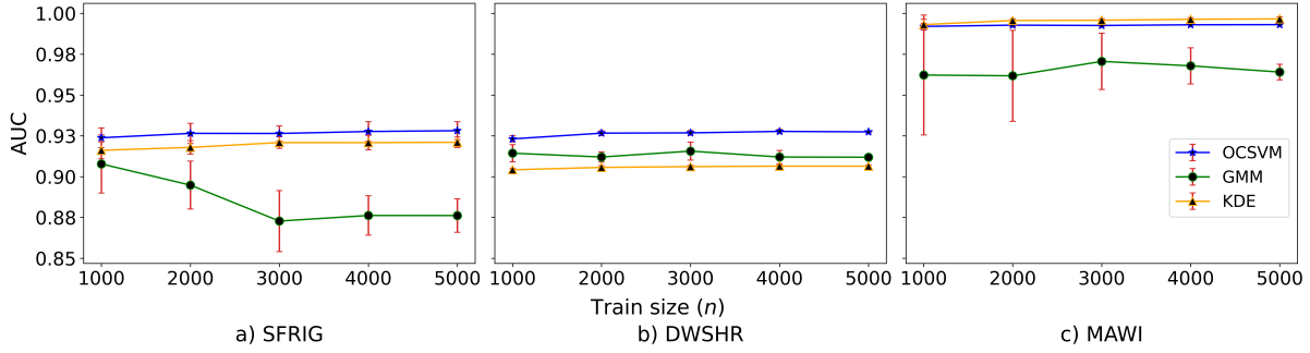
Figure 1: Detection performance of OCSVM vs that of GMM and KDE on two IoT datasets (a and b), and on general purpose PC (c). OCSVM’s remain competitive against these other classical and flexible methods.
