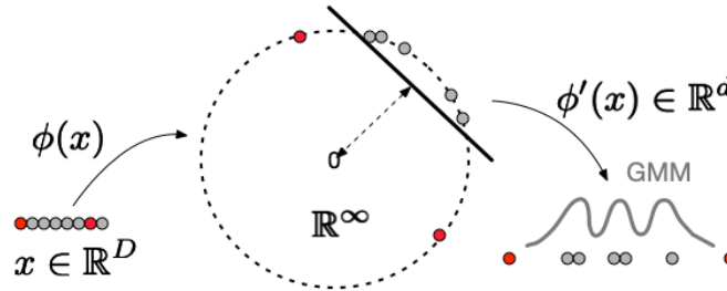
Figure 2: OCSVM maps datapoints x \in \mathbb{R}^D as \phi(x) onto a ball in \mathbb{R}^\infty , inducing linear separation between normal points (gray) and yet unseen novel points (in red). We consider mappings \phi' which then remap down to \mathbb{R}^d , d \ll D , while maintaining separation (into clusters), but not necessarily linear separability. Given the few modalities of IoT devices, we can then learn a GMM with few components to model the remapped normal data.
