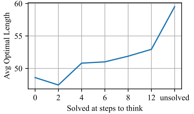
Figure 3. Average optimal solution length of levels grouped by the number of thinking steps at which the level is first solved. Each of the 50,000 medium-difficulty validation levels is assigned to a group.
