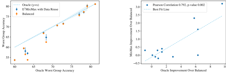
(a) Comparing non-parametric group DRO methods
