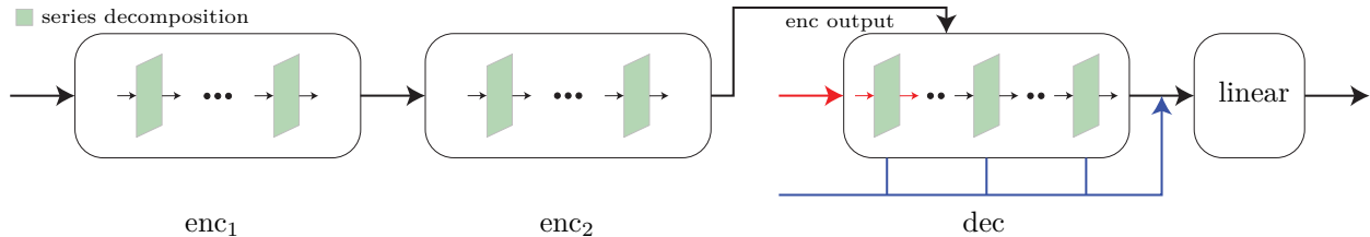
Figure 1: We study Transformer-based architectures (Wu et al., 2021; Zhou et al., 2022) that include two encoders and one decoder, and an output linear layer. We sample geometric features in sequence decomposition layers, depicted as small rectangles within the blocks.
