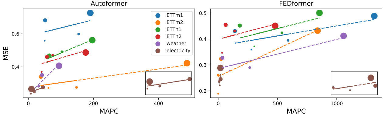
Figure 5: MAPC is correlated with model performance. The test mean squared error is proportional to the MAPC on multiple datasets. Due to different scales, an inlay of the electricity data set is added to the bottom right corner of each architecture.
