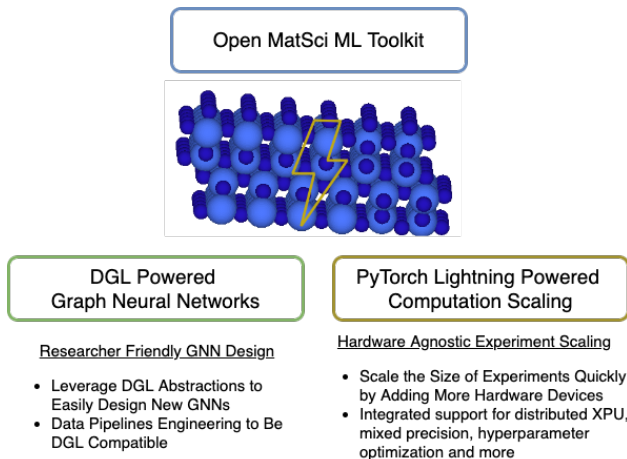
Figure 1: Open MatSci ML Toolkit enables researchers to create and perform scientific machine learning on the OpenCatalyst in a scalable manner leveraging DGL and PyTorch Lightning.
