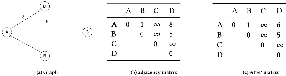
Figure 2: Graph, adjacency matrix, and APSP matrix, after removing node C.
