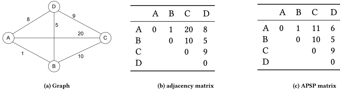
Figure 1: Graph, adjacency matrix, and APSP matrix.
