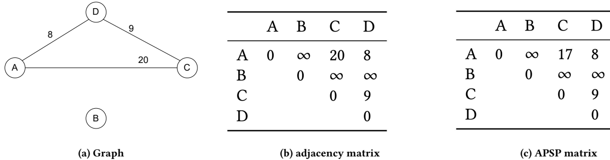
Figure 3: Graph, adjacency matrix, and APSP matrix, after removing node B.
