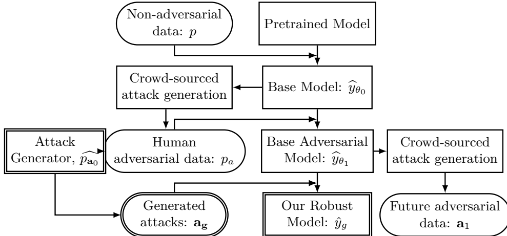
Figure 1: The framework that shows how each dataset and model is created. Our contributions are double lined. Not pictured: \hat{y}_g is then evaluated on the future real attacks, \mathbf{a}_1
