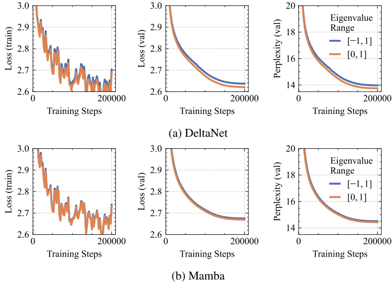
Figure 7: Learning curves of Mamba (370M) and DeltaNet (340M) when training on 32B tokens of Fine-Web 100B.
