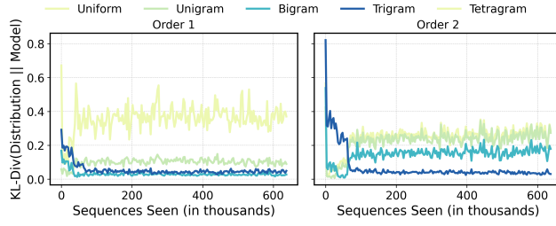
Figure 2: A transformer trained on sequences generated by random order-1 and order-2 Markov chains can infer whether the context is order-1 or order-2, then generate predictions using the corresponding bigram or trigram statistics. (Left) shows the distance between the model’s output distribution on the last token and well-defined context strategies for order-1 inference, as a function of the number of sequences seen during training. (Right) presents analogous results for order-2 inference.
