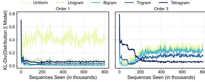
Figure 1: We train a transformer for next-token prediction on sequences generated by random order-1 and order-3 Markov chains. During inference, we assess its ICL ability by evaluating performance on sequences derived from unseen order-1 and order-3 chains. (Left) shows the distance between the model’s output distribution on the last token and n -gram statistics of the context for order-1 inference, as a function of the number of sequences seen during training. (Right) presents analogous results for order-3 inference. Notably, the trained transformer can identify the true order (1 or 3) of the context, and then predict using either bigram or tetragram statistics accordingly.
