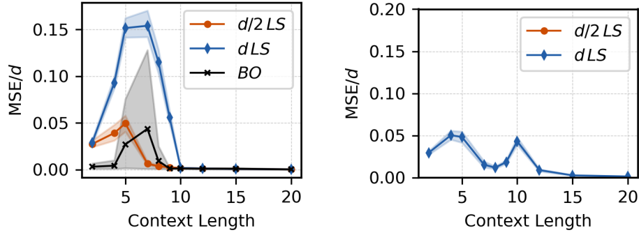
Figure 7: Replicating the experiment in Fig. 3 using d = 10 .
