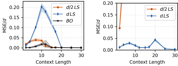
Figure 3: A transformer trained on X = [\mathbf{x}_1, y_1, \mathbf{x}_2, y_2, \dots, \mathbf{x}_T, y_t] sequences generated using random d -dimensional and d/2 -dimensional regressors (see Section 3 for details). We plot (M_\theta([X, \mathbf{x}_{\text{test}}]) - \mathbf{w}_{\text{bench}}^T \mathbf{x}_{\text{test}})^2 / d where \mathbf{w}_{\text{bench}} refers to two benchmark least-squares solutions in d or d/2 dimensional space described in Section 3. When prompted with sequences from unseen d/2 (left) or d dimensional regressors (right), the transformer’s predictions align most closely with the corresponding LS solution \mathbf{w}_{d/2}^{\text{LS}} or \mathbf{w}_d^{\text{LS}} . Here, d = 20 and training context length T = 39 . See App. for a similar experiment with d = 10 .
