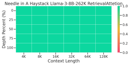
Figure 5: Performance of RetrievalAttention in Needle-in-a-haystack.
