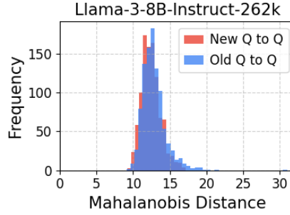
Figure 9: The Mahalanobis distance from the newly generated queries (New Q) and sampled prefill queries (Old Q) to the remaining prefill queries.
