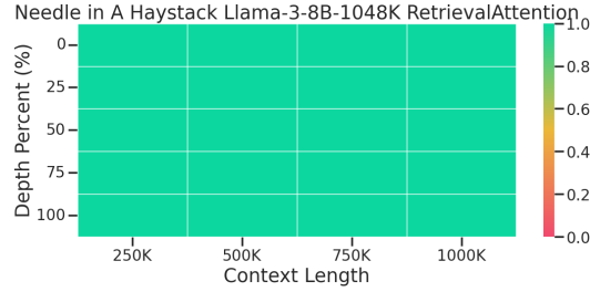
Figure 8: Performance of RetrievalAttention in 1 million Needle-in-a-haystack test.
