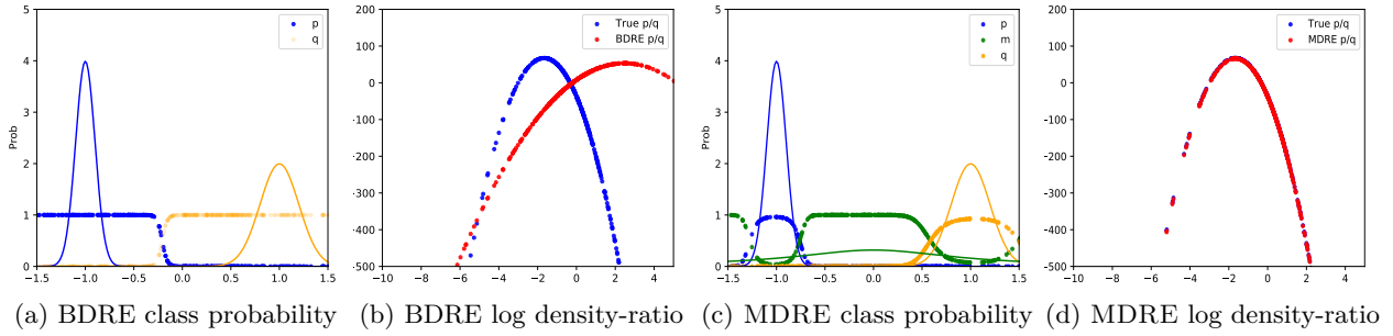
Figure 1: BDRE vs proposed MDRE on estimation of log density ratio where p = \mathcal{N}(-1, 0.1) and q = \mathcal{N}(1, 0.2) . For MDRE, the auxiliary distribution m is Cauchy \mathcal{C}(0, 1) . Plots (a) and (c) show the class probabilities P(Y|x) learned for BDRE and MDRE respectively overlaid on the plots of p , q and m . Plots (b) and (d) show the estimated log density-ratio by BDRE and MDRE respectively. Using auxiliary distribution m allows MDRE to better estimate the log density-ratio.
