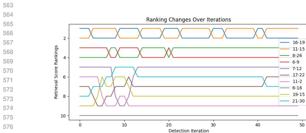
Figure 13: Illustrate how Ranking of top retrieval heads of Llama2-7B-80K changes when detection iteration increase.
