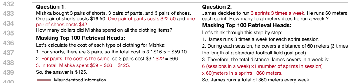
Figure 11: When we mask out retrieval heads, the model ignores important information in the question description resulting in incorrect reasoning chains.
