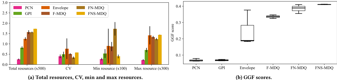
Figure 6: Performances of multi-policy MORL baselines and our methods in resource gathering ( D = 3 ).
