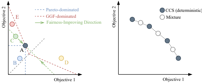
Figure 3: Left Figure: Point A is always preferred to B due to Pareto dominance; A is always preferred to C due to the Pigou-Dalton transfer principle (fairer solution); depending on the weights of GGF, Points D and E can be dominated or non-dominated by A (w.r.t. GGF); with weights (0.3, 0.7), A is preferred to E but not to D. Right Figure: Black points refer to deterministic policy that in CCS and stochastic policy can be obtained with the mixture of deterministic policies in the CCS, shown in dotted point. Demonstrate that stochastic policy may achieve a fairer solution, which deterministic policy cannot.
