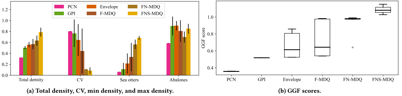
Figure 4: Performances of multi-policy MORL baselines and our methods in species conservation ( D = 2 )
