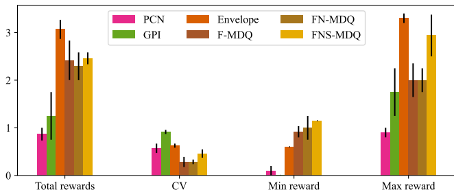
(a) Total rewards, CV, min reward, and max reward.
