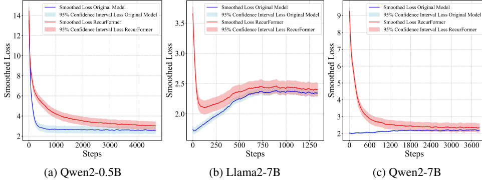
Figure 3: Loss values of RecurFormer and the corresponding original models during continual training on the masked prediction task using the Wikipedia English training set.
