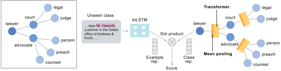
Figure 1: Left: A sample from the 2-hop neighbourhood for the concept lawyer from ConceptNet. Right: The ZSL-KG architecture. The text with the named-entity is passed through the example encoder (biLSTM with attention) to generate the example representation. For the class representation, we take the k-hop neighbourhood and pass the nodes through their hop-specific transformer graph convolutional network (TrGCN). The same architecture is used for language tasks with a task-specific example encoder.
