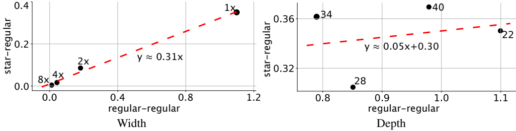
Figure 3: “Starness” vs. model width and depth. For starness vs. model width (left), we vary the width of a WideResNet (depth 22) from 1\times to 8\times . For starness vs. model depth, we vary the depth of a WideResNet (width 1\times ) from 22 to 40 layers. For each depth-width combination, we plot the loss barriers B(\theta^*, \theta_h) between star models \theta^* and heldout models \theta_h \in H on the y-axis. As a reference point, we plot the barrier between two regular solutions B(\theta_A, \theta_B) , on the x-axis. The points are annotated with the corresponding widths or depths. Star models consistently enjoy better linear connections with regular models, than do the regular models amongst each other.
