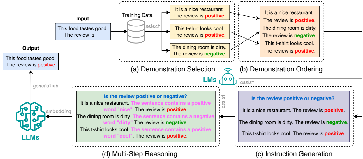
Figure 19: Illustrations of few-shot prompting techniques for LLMs.
