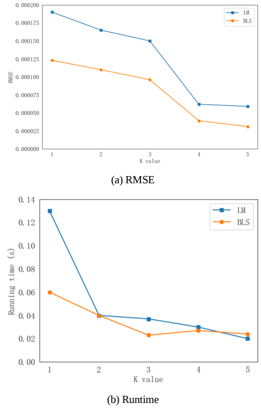
Fig. 8. Results comparison in category C
