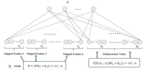
Fig. 4. Feature and Enhancement layers of BLS
