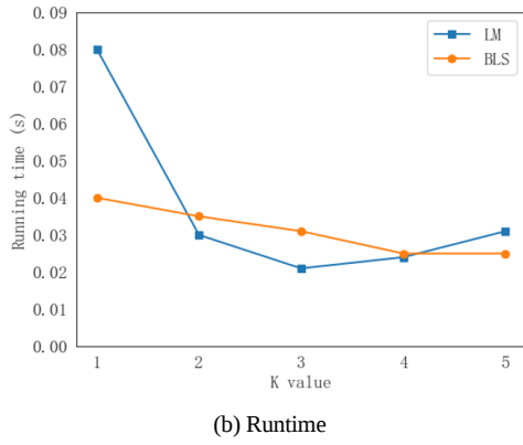
Fig. 6. Results comparison in category A
