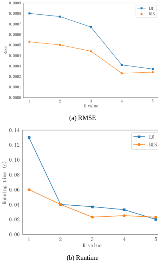
Fig. 7. Results comparison in category B
