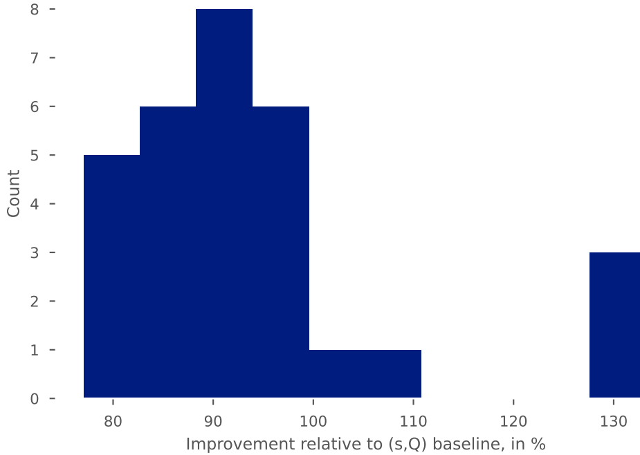
Figure 2: Improvement of GLDQN over (s, Q) -policy, for the H = 2 scenario, for 30 generations of 100 items.
