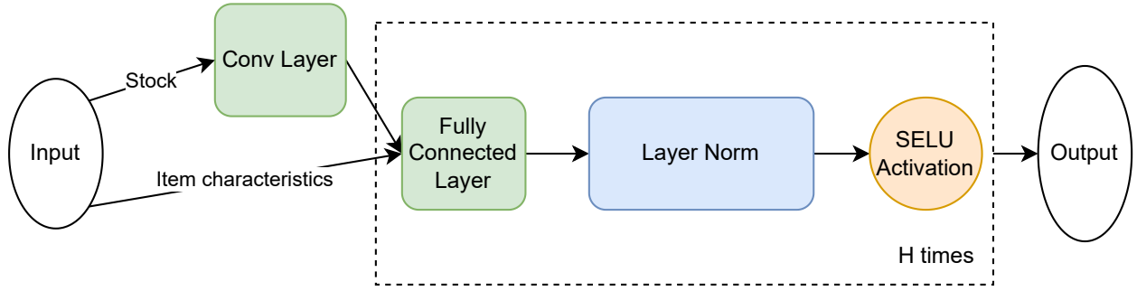
Figure 1: Neural architecture for all DQN-based models
