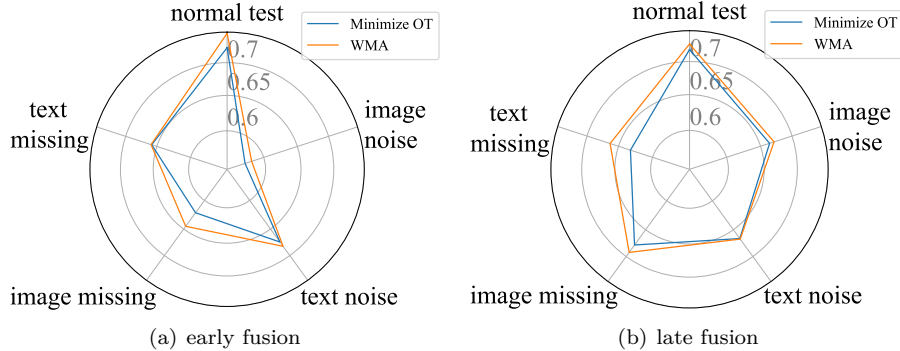
Figure 4: Results of our proposed method with minimizing OT distance on Hateful Memes datasets. See the result for all datasets in Table 11 and Table 12.
