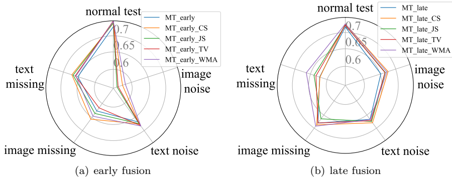
Figure 5: Results of our proposed method with different distance metrics on Hateful Memes datasets. See the result for all datasets in Table 13 and Table 14.
