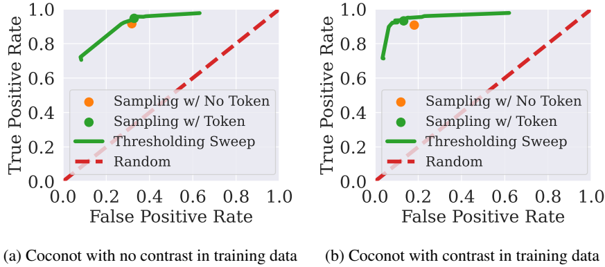
Figure 2: Manipulating the refusal token provides different refusal rates at test-time without retraining. The left and right figures show that both true positive and false positive rates on coconot eval change as we vary the threshold of the refusal token. The models are trained with ultrachat and refusal messages from the coconot training data. Left is trained without any contrast data, and the right is trained with contrast data, which is one-tenth of the refusal data. All refusal and training are from the coconot training data.
