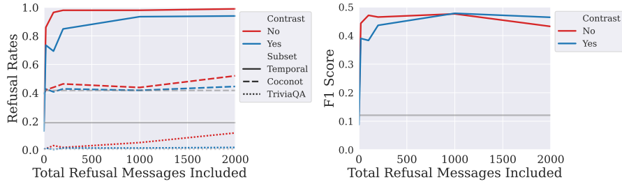
Figure 8: Left are refusal rates on the three subsets of the evaluation: temporal questions, coconot questions, and TriviaQA questions where one model is trained with contrast data and one without. Right are F1 scores. The x-axis is how many instructions the model was trained with. The gray line represents the rates with no refusals messages in the instruction data and both are trained with the refusal token. From these plots, the contrast data plays an important role when scaling the amount of data up and limits the Type II error.
