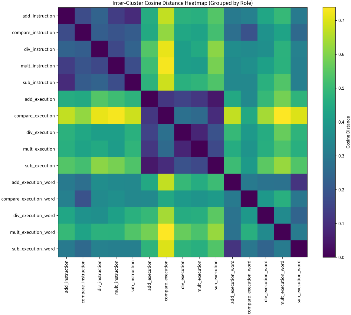
Figure 4: Cosine distances between cluster centroids for each operation-role pair, grouped by role: instructional texts (top block), execution strings (middle), and worded executions (bottom). Each centroid represents the average embedding of 50 samples per category, computed using LLaMA2-7B-chat. Clear geometric separation is observed between instructional and execution-related forms, with execution and worded execution clusters being closer to each other than either is to instruction. This provides quantitative support for the hypothesis that instruction-following and execution are learned as distinct representational pathways within the model’s embedding space.
