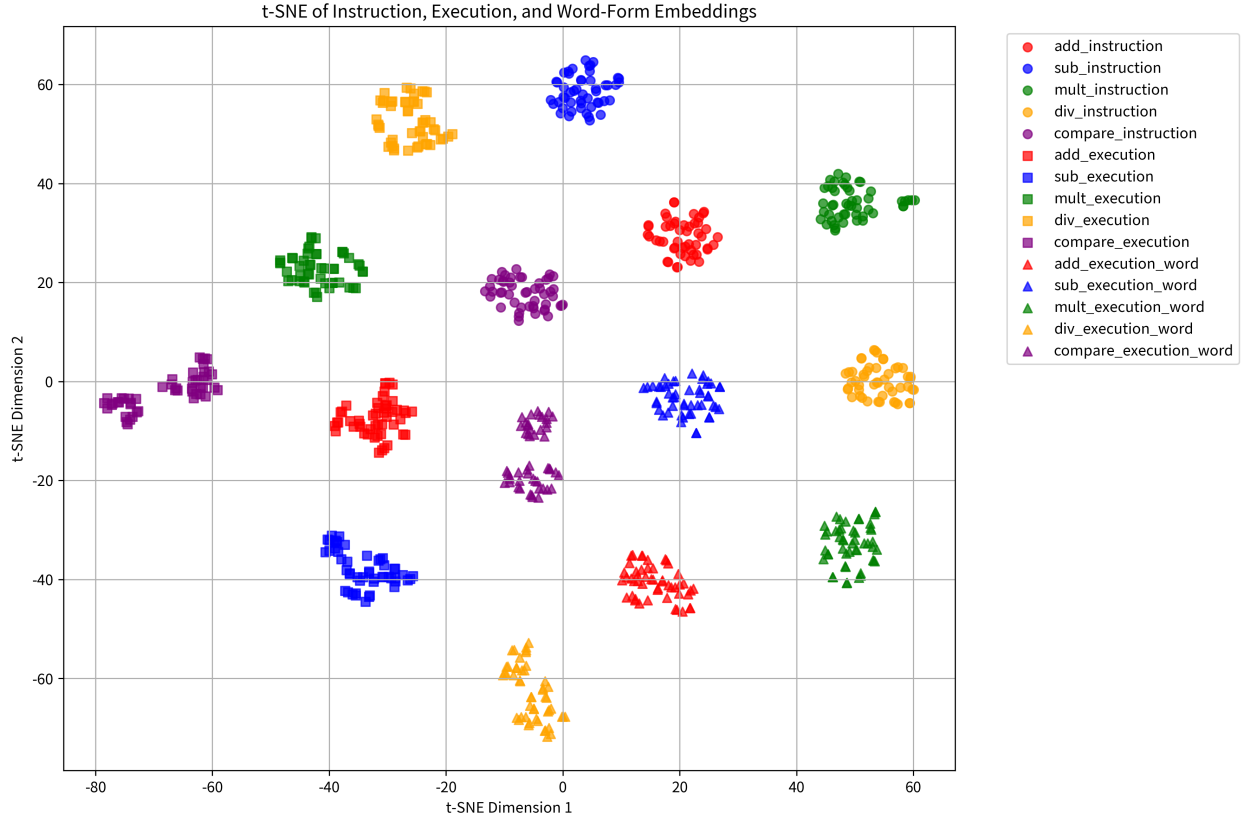
Figure 3: t-SNE projection of instruction, symbolic execution, and word-form execution embeddings from LLaMA2-7B-chat, across 50 problems each in five arithmetic operations. Instructions (circles), symbolic expressions (squares), and word-form results (triangles) occupy geometrically distinct regions, despite describing the same operation. This illustrates that LLaMA2-7B-chat stores instructional knowledge and executional know-how in separate regions of its latent space.
