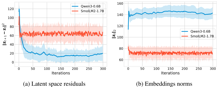
Figure 17: LLM models can induce well-behaved latent vector fields: For latent space iterations in Qwen3-0.6B and SmoLM2-1.7b, we plot the latent residuals norms(a); and norms of embeddings across iterations (b).
