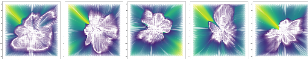
Figure 1: Latent dynamics of AEs . Latent vector fields induced by autoencoders with bottleneck k = 2 , trained on MNIST, with \mathbf{z}_0 \sim \mathcal{U}[-8, 8] . Models with different initializations are shown. Colors (viridis colormap) represent vector norms ranging from violet (low) to yellow (high). The shape of the latent manifold identifies with the encoder’s support. White regions indicate where the vector field vanishes, revealing attractors aligned with high-density areas of the data distribution.
