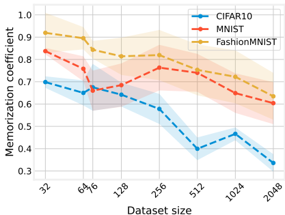
Figure 14: Strong overparametrization favors memorization : Memorization coefficient as a function of the dataset size on CIFAR, MNIST, FashionMNIST, showing that networks trained on less data (strongly overparametrized) tend to memorize more the training data.
